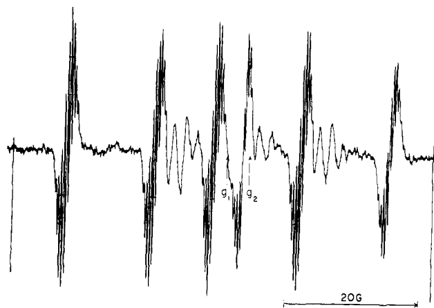
Figure 1. Esr spectrum of a mixture of 2,4,6- tert -butylphenyl isopropyl nitroxide and N -isopropoxy-2,4,6- tert -butylanilino radical in benzene solution at 2.5 hr after spin trapping. Arrows in spectrum indicate center of each: g_1 = 2.00602 , g_2 = 2.00402 .
